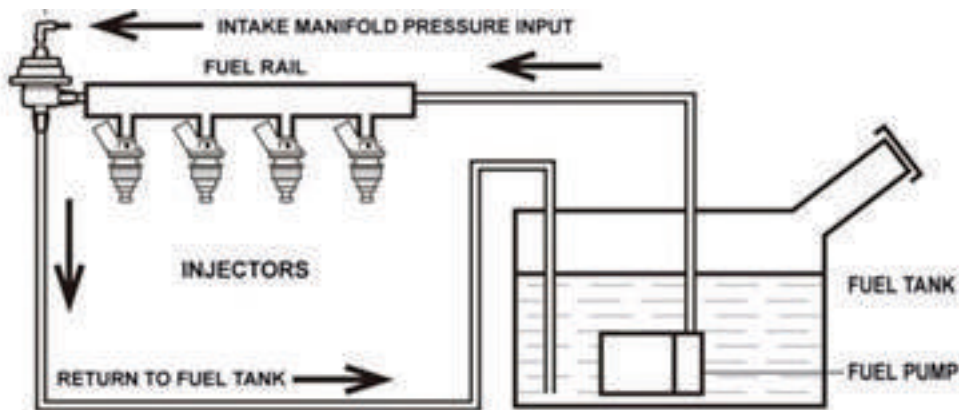
GENERAL FUEL SETUP SYSTEM EXAMPLE
